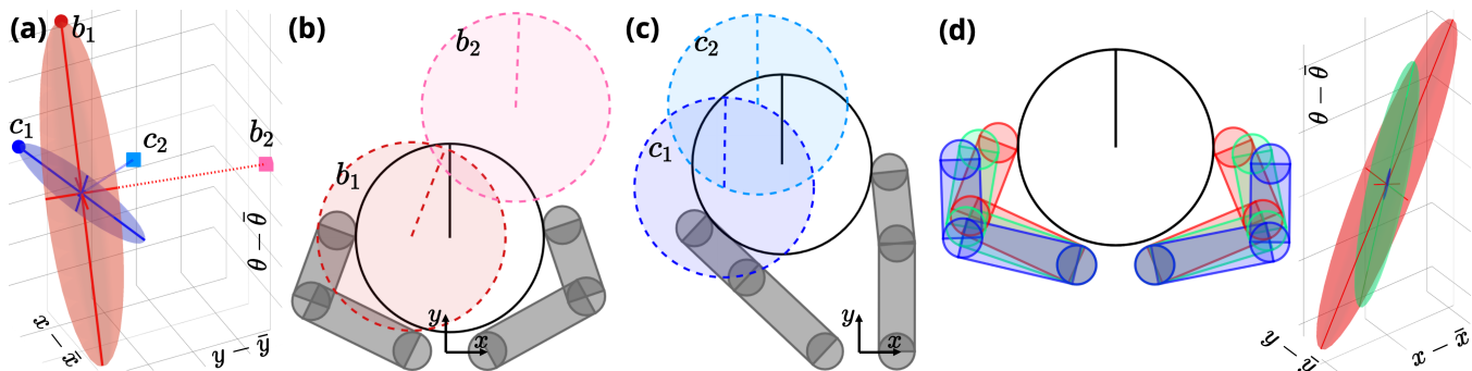
Fig. 8: (a) Two different sublevel sets \mathcal{R}_{\rho, \epsilon, \gamma}^u , represented as ellipsoids, shown in the space of q^u , with \epsilon = 1 , and \gamma = 10^{-6} . The ellipsoid centers are shifted to the origin for easy comparison. Red ellipsoid: \mathcal{R}_{\rho, \epsilon, \gamma}^u for the system configuration in Fig. 8b; blue ellipsoid: \mathcal{R}_{\rho, \epsilon, \gamma}^u for the configuration in Fig. 8c. Points b_1, c_1 are where ellipsoids' major axes intersect their boundaries. Points b_2, c_2 are points along the minor axes of the ellipsoids, and satisfy \|b_1\| = \|b_2\| and \|c_1\| = \|c_2\| , where the norm is based on the standard Euclidean metric. (b) The solid robots and objects represent the \bar{q} at which the red \mathcal{R}_{\rho, \epsilon, \gamma}^u in (a) is computed. The straight line on the puck indicates its orientation. The dashed dark red puck corresponds to the configuration b_1 , and pink to b_2 . Note that b_1 is easier to reach than b_2 . (c) Similar to Fig. 8b, the dashed dark blue puck correspond to c_1 , and light blue to c_2 . It is also easier to reach c_1 than c_2 . (d) The volume of \mathcal{R}_{\rho, \epsilon, \gamma}^u shrinks as the fingers get further away from the puck. The ellipsoids on the right are color-coded to match the robot configurations on the left. Note that the blue ellipsoid is barely visible.
