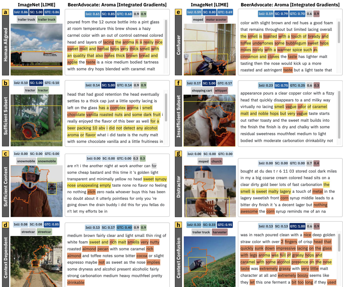
Figure 3: Using Shared Interest we identify eight recurring patterns in model behavior across two domains and saliency methods: an ImageNet [10] classification model with LIME [34] and a BeerAdvocate sentiment regression model [7, 25, 27] with Integrated Gradients [7, 41]. Each example includes the IoU, GTC, and SC scores, true label (grey), and model prediction (green if correct, red otherwise). Ground truth features are highlighted in yellow and saliency features are highlighted in orange.
