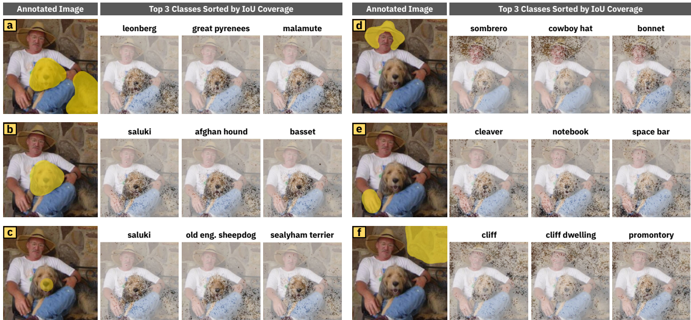
Figure 7: Shared Interest enables users to probe the model with different ground truth features to understand model behavior. By comparing the user’s annotation (shown in yellow) to the saliency feature set (shown via saturation) for every ImageNet class, Shared Interest surfaces the classes most related to the annotated features. Probing with smaller and smaller sets of features (a-c) shows the model has learned characteristic features of dogs. Probing with secondary objects (d) demonstrates that the model learns about objects other than the labeled object in the image. Probing the model with features it has not learned to classify (e) indicates the model learns to relate these features to associated objects (e.g., hand and cleaver). Finally, probing with background features (f) demonstrates that the model has learned related features despite only being trained on foreground classification.
