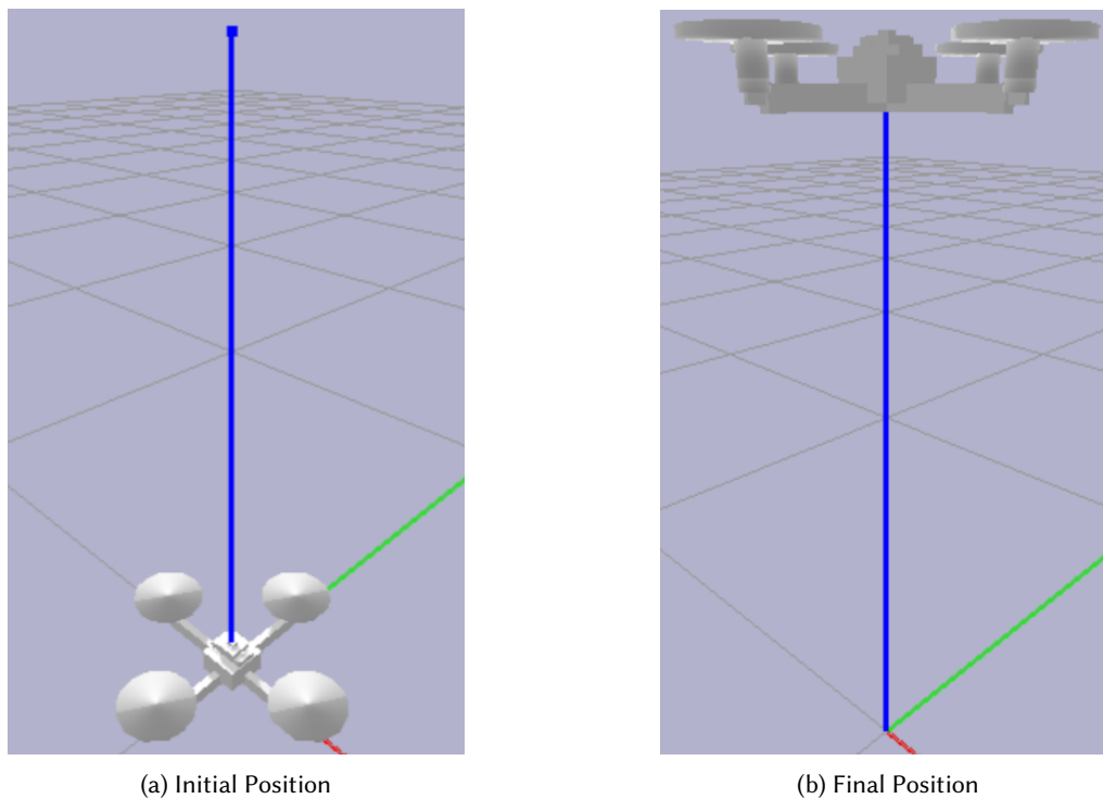
Fig. 81. Simulating Quadcopter Performance. Left: Following the OpenJSCAD to URDF conversion script provided by GPT-4, we show the quadcopter rendered in PyBullet's simulator. The quadcopter has optimized frame bar lengths discovered with the script provided by GPT-4 and is resting at its initial position. Right: Using the LQR controller designed by GPT-4, the quadcopter is able to lift off and hover at the goal position 1m off the ground.
