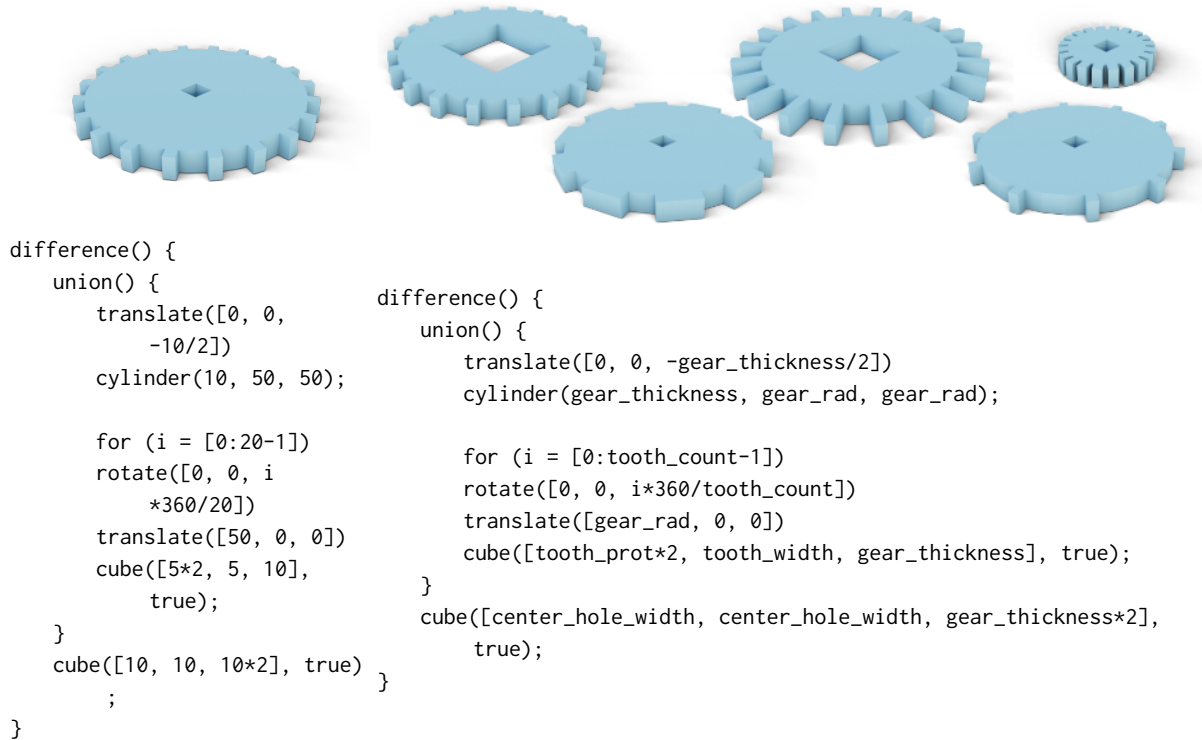
Fig. 21. Gear Design Space. The same gear ( Top left ) can be constructed with different design representations. Here, we have an OpenSCAD design ( Bottom left ) and a parametric OpenSCAD design ( Bottom right ) where the degrees of freedom ( Top right ) have been exposed via design variables.
