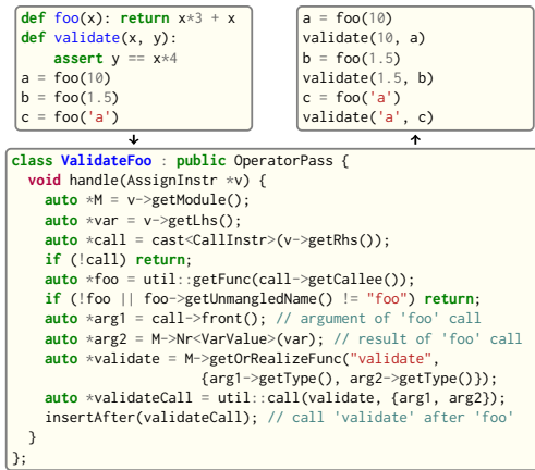
Figure 3. Example of bidirectional compilation in Codon IR. The simple pass, shown in the bottom box, searches for calls of function foo , and inserts after each a call to validate , which takes foo ’s argument as well as its output and verifies the result. Both functions are generic and can take as an argument any type that can be multiplied by an integer, so the type checker is re-invoked to generate three distinct validate instantiations for the example code in the top left box, producing code equivalent to that in the top right box.
