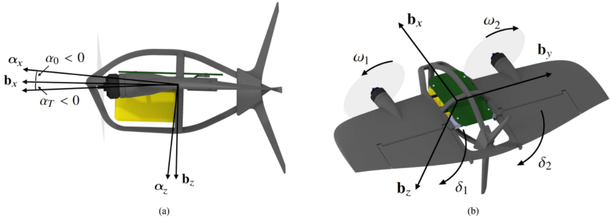
Fig. 2. Reference frame and control input conventions. The green board is mounted toward the top of the wing; the yellow battery toward its bottom. (a) Zero-lift reference frame, zero-lift angle of attack, and thrust angle. (b) Body-fixed reference frame, and control inputs, i.e., rotor speeds \omega_1 and \omega_2 , and flap deflections \delta_1 and \delta_2 .
