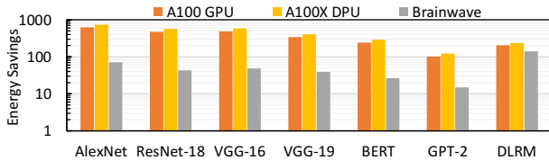
Figure 22: [Simulation] LIGHTNING’s average energy consumption savings compared to state-of-the-art accelerators.
