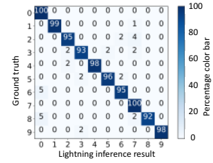
Figure 16: [Testbed] LeNet inference accuracy on LIGHTNING.
