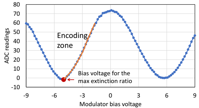
Figure 23: Sweeping the modulator bias voltage to find the max extinction ratio for LIGHTNING.
