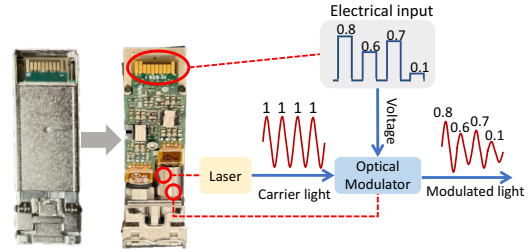
Figure 1: Amplitude modulation in a commodity transceiver.
