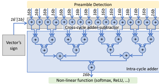
Figure 10: Pipeline parallel digital adder module.
