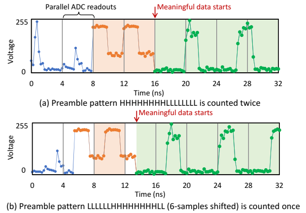
Figure 9: Preamble pattern distinguishes noise from data.
